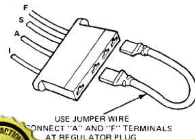
FIG. 2 Field Circuit Test
