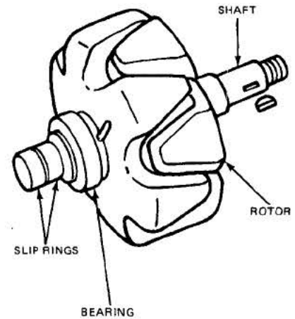
FIG. 9 Rotor Assembly—Typical
