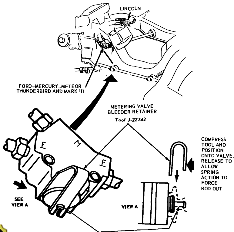
FIG. 14—Master Cylinder Installation—Lincoln Continental
