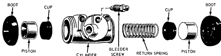
FIG. 5—Brake Wheel Cylinder—Typical
